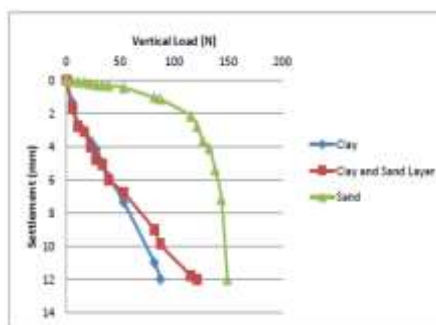
Fig. 4. Vertical load – Settlement curve of single pile for varying soil medium for L/D ratio 24
