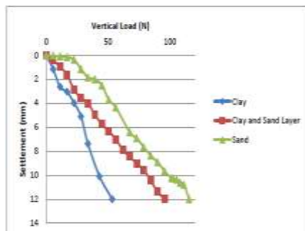
Fig. 3. Vertical load – Settlement curve of single pile for varying soil medium for L/D ratio 12
