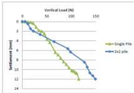
Fig. 7. Vertical load – Settlement curve for number of piles (L/D Ratio=12) in Sand
