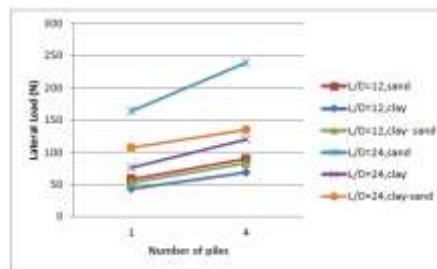
Fig. 14. Lateral Load – number of piles variation of piles for different soil medium and L/D ratio for 25 mm deflection
