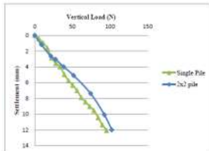
Fig. 9. Vertical load – Settlement curve for number of piles (L/D Ratio=12) in Clay- Sand Bed
