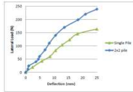
Fig. 12. Lateral load – Deflection curve for varying number of piles (L/D Ratio=24) in Sand
