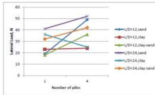
Fig. 15. Variation of Lateral Load – Number of piles for different soil medium and L/D ratio at 4.5mm deflection
