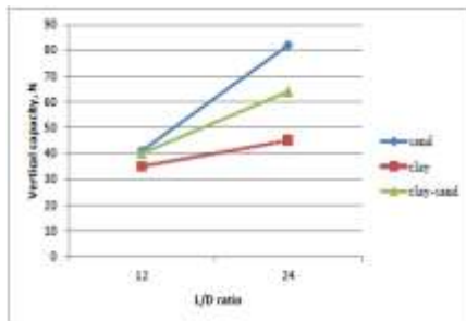
Fig. 5. Vertical Load – L/D Ratio variation of single pile for different soil medium at 6mm settlement
