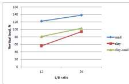
Fig. 6. Vertical Load – L/D Ratio variation of 2x2 pile group for different soil medium at 6mm settlement
