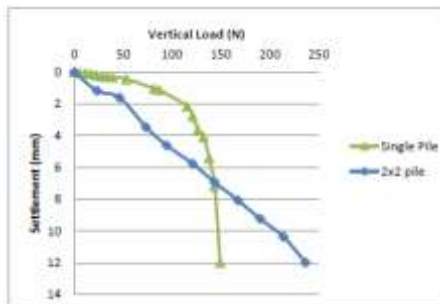
Fig. 10. Vertical load – Settlement curve for number of piles (L/D Ratio=12)
