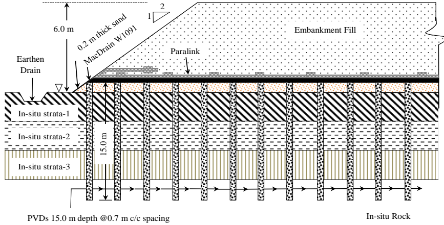
Fig. 1. Typical cross section (a portion of the total embankment width of 106 m) of railway track (Ch-03+900 to Ch-04+400 km)
