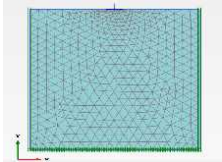
Fig. 3. Model generation in Plaxis- 2D
