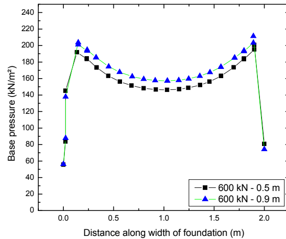
Fig.5. Base pressure distribution for isolated footing with 600 kN loading on lacustrine clay from PLAXIS 2D analysis
