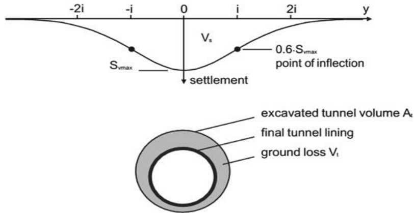
Fig. 1. Gaussian Curve for Settlement in presence of void [6]
