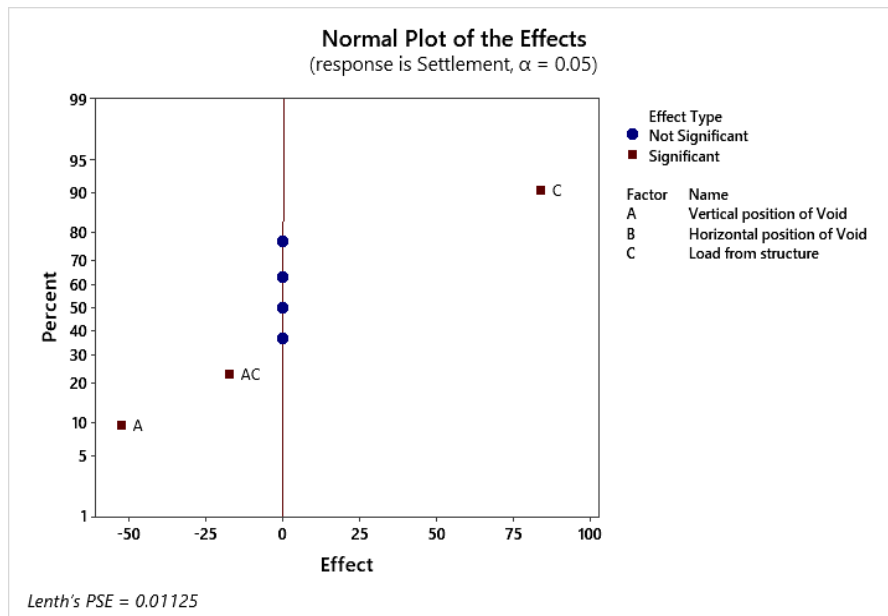
Fig. 7. Effects of various factors and their interrelations
