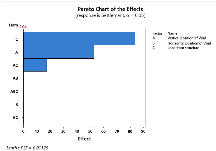
Fig. 8. The Pareto Chart of the effects
