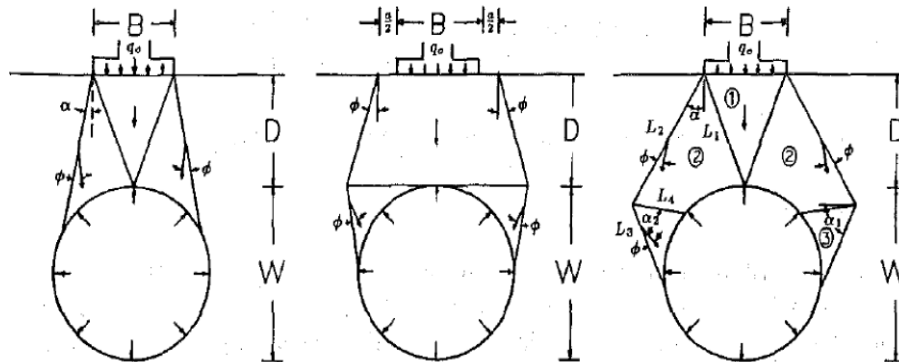
Fig. 2. Failure mechanism of footing collapse [10]
