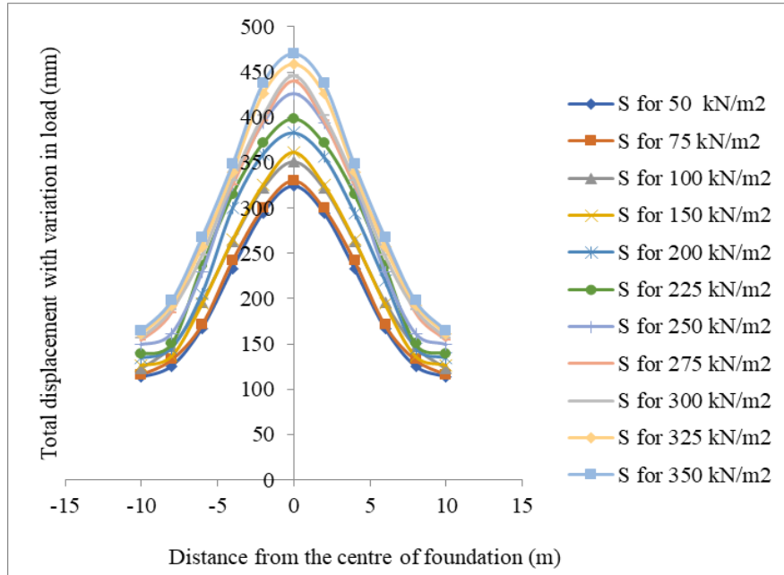
Fig. 6. Variation of total displacement with the distance from the centre of the foundation with a change in load
