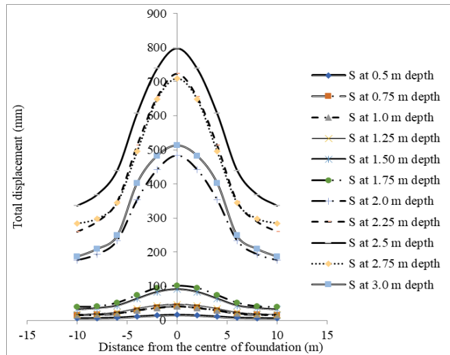
Fig. 5. Variation of total displacement with the horizontal distance from the centre of the foundation
