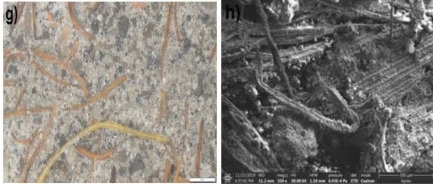
Fig. 2. Stereomicroscopic and SEM images of a-b) Untreated soil, c-d) AAB treated soil, e-f) PF-AAB treated soil, g-h) TCF reinforced AAB soil.
