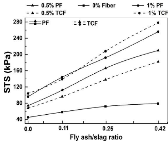
Fig. 4. Variation of STS for PF and TCF reinforced AAB treated soil at different fiber dosages.
