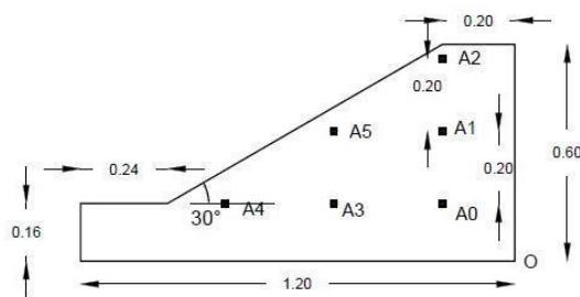
Fig. 2. Locations of the sensors in the model and the SEN0114 soil moisture sensor
