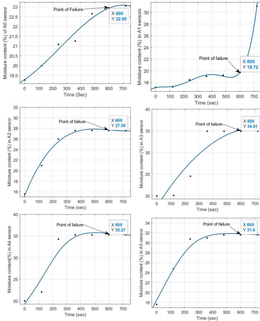
Fig. 6. Moisture content vs Time graph of each sensors in the 60° slope model
