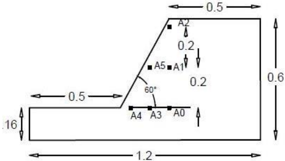
Fig. 5. Locations of the sensors (not to scale)
