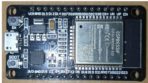
Fig.7. ESP32-WROOM-32 Micro-controller
