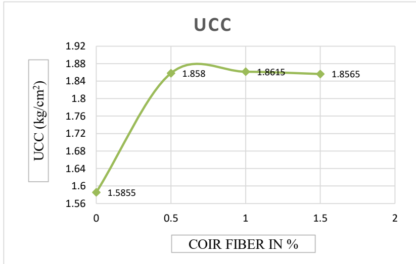
Fig.5. UCC for soil stabilized with coir fiber (pore fluid is water)
