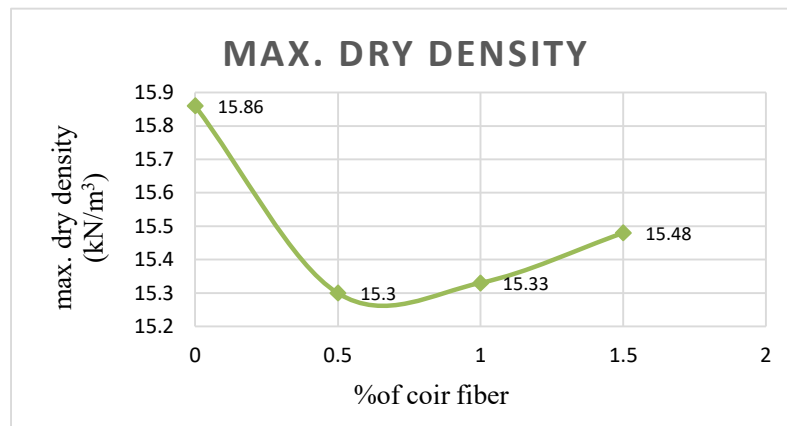
Fig. 3. Variation of Maximum dry density for coir stabilized soil.
