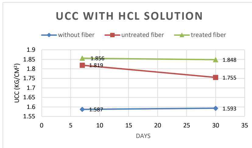
Fig.6. UCC for HCL solution as pore fluid.
