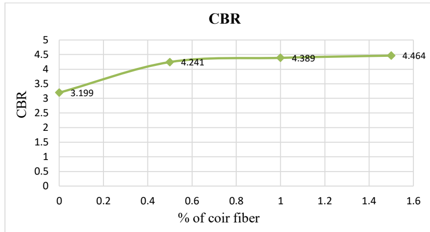
Fig.4. CBR for soil stabilized with coir fiber
