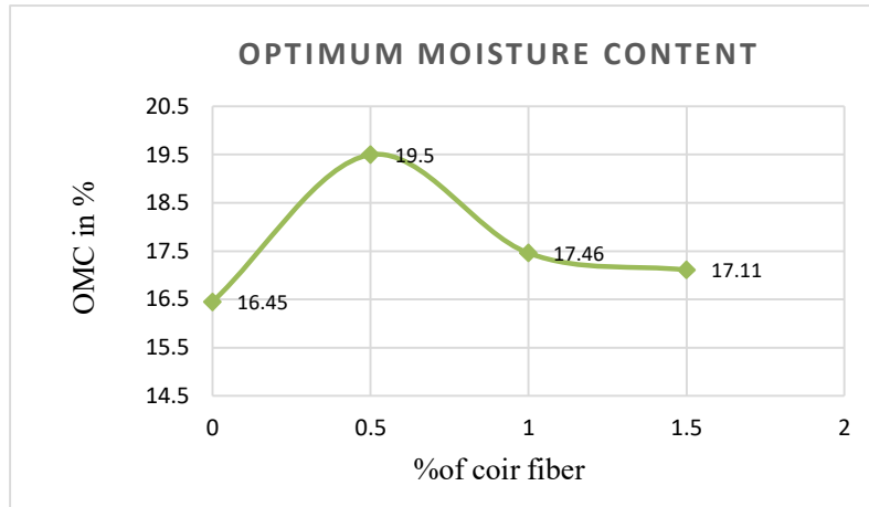
Fig. 2. Variation Optimum moisture content for coir stabilised soil
